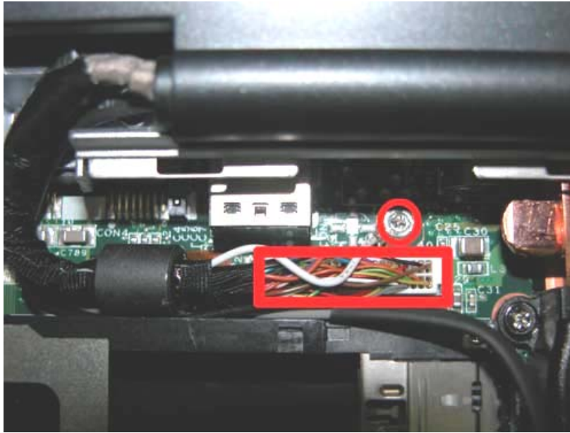
Fig. 15 Removing screws retaining LCD Cable Connector
